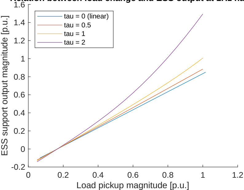
Relation between load change and ESS output at 1Hz nadir
